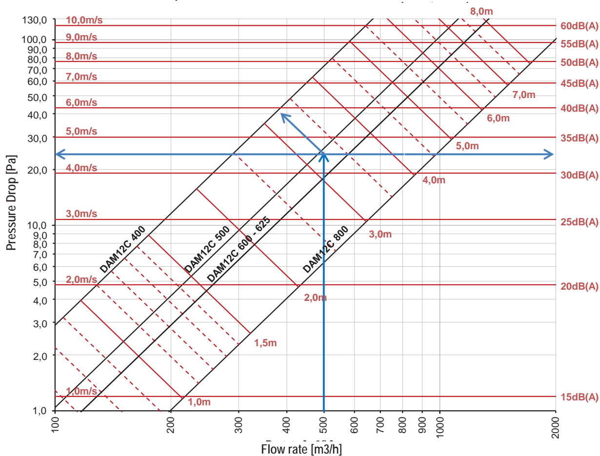
Flow Rate / Pressure Drop Air Outlet Speed / Noise Level / Horizontal Throw (Vt.: 0,25m/s)
